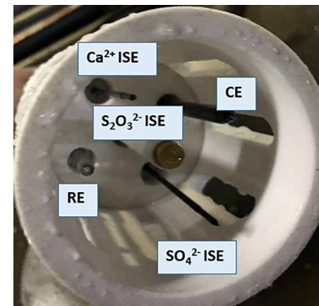
Figure 21 and 22. Electrochemical Sensor System
