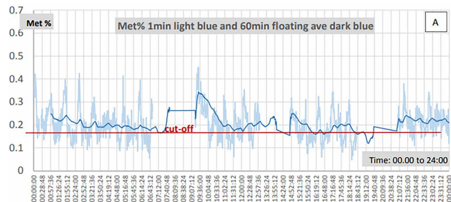
Figure 3. The study on metal content (%) during 24 hours shows 1 minute (light blue) and 60 min (dark blue) floating average rate from primary crushed ore [8].
