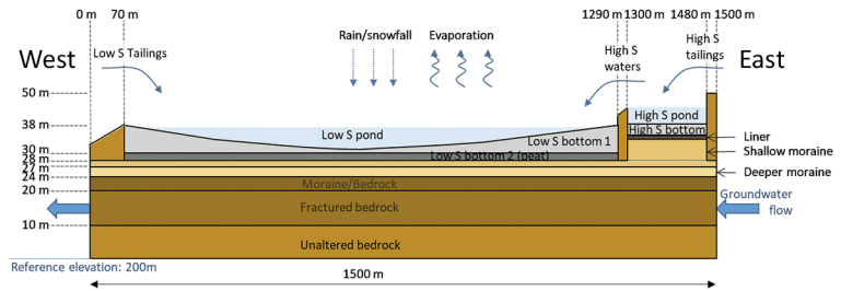
Figure 27. Cross-section of the modelled system for the Finnish mine highlighting the different hydrogeochemical units and the various types of fluxes
