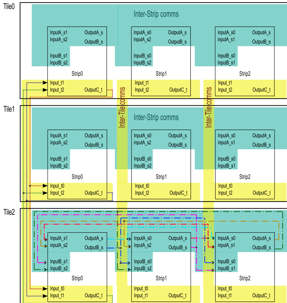
Figure 4.4 – A 3x3 Fynbos array providing a representation of the data sharing interconnect only. Inter-Tile communication lines appear for the first column of strips only, similarly the inter-strip communication lines are shown in Tile2 only. In both cases for clarity the remaining interconnect lines are indicated as shading otherwise. In summary, within a Tile two data words are made available from each Strip to every other Strip within the same Tile, between Tiles one data word is made available to every other Tile’s column index corresponding Strip.
